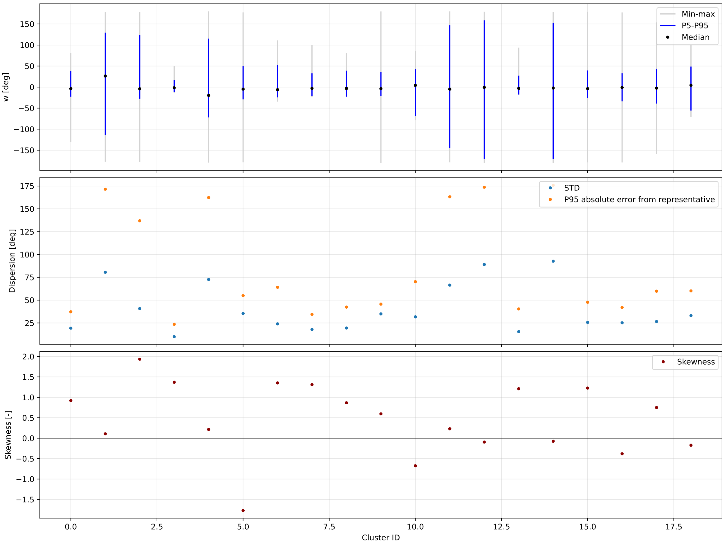
K=19 | forward | w | valid=194058/194058 | offsets from each cluster circular mean
