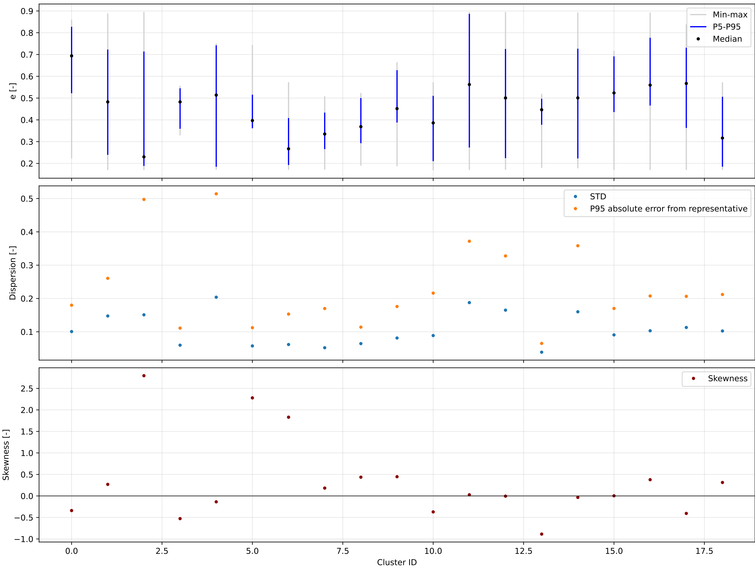
K=19 | forward | e | valid=194058/194058
